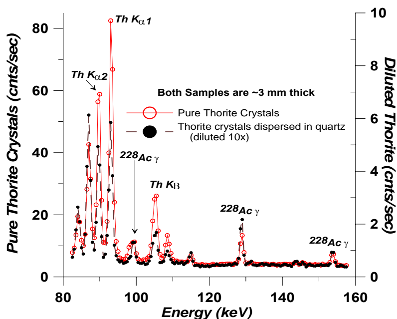
Figure 4. A comparison of emission spectra collected from concentrated and diluted Th samples. When pure thorite crystals are analyzed (sample thickness = ~3 mm), the intensity of the Th K \alpha and Th K \beta emissions are higher relative to the amount of Th or total radioactive decay than for a sample where Thorite is diluted (10 x) and more finely dispersed. Further evidence that Th fluorescence contributions are significant in the more concentrated Th sample is given by the ratio of the 90 keV K \alpha 2 line to the 93 keV K \alpha 1, which approaches the more expected ratio ~0.6. In more diluted Th samples, the ratio of the 90 keV to 93 keV is closer to 1 (See also Figure 1), because the relative importance of typical decay emissions, particularly at 90 keV, dominates the spectra rather than fluorescence. In the case of the pure thorite spectrum, natural Th fluorescence could interfere with quantifying the 92-93 keV ^{234}\text{Th} gamma doublet.
