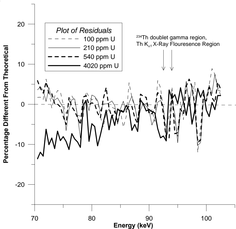
Figure 3. Plot of residuals in the 70-105 keV range for Th and U mixtures: [measured spectra – theoretical spectra]. The amount of Th in the samples remained constant at 0.12 g (all mixtures = 732 ppm Th). Theoretical spectra were calculated by summing the appropriate fractions of the spectra of the U and Th parts given in Figures 1 (plot +) and 2).
