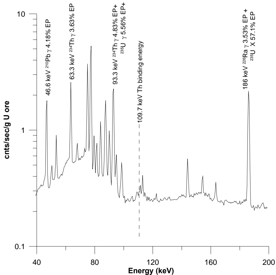
Figure 2. Emission spectrum collected from a U ore sample (diluted with quartz).
